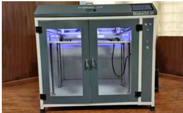
CENTRE FOR SMART MANUFACTURING 3D PRINTER 500MM X 500MM X500MM
